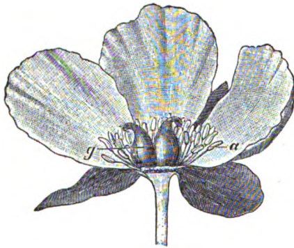
FIG. 183. — A typical flower, of Peonia peregrina ; \times \frac{1}{2} .
